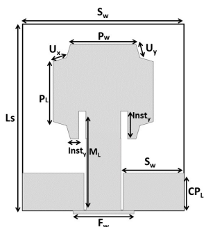
Fig. 2. Antenna Layout
